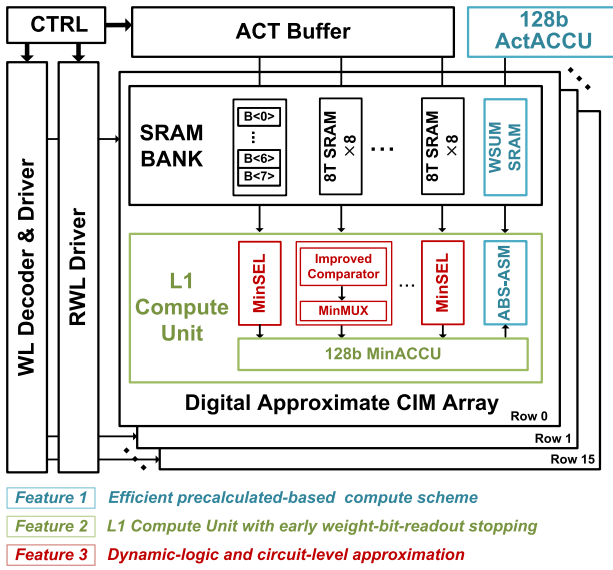
Fig. 5. Overall architecture of multiply-less approximate CIM macro.
