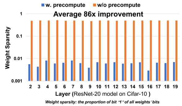
Fig. 7. Weight sparsity gains due to the precomputation.
