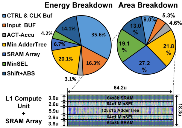
Fig. 16. Energy and area breakdown of test-chip.
