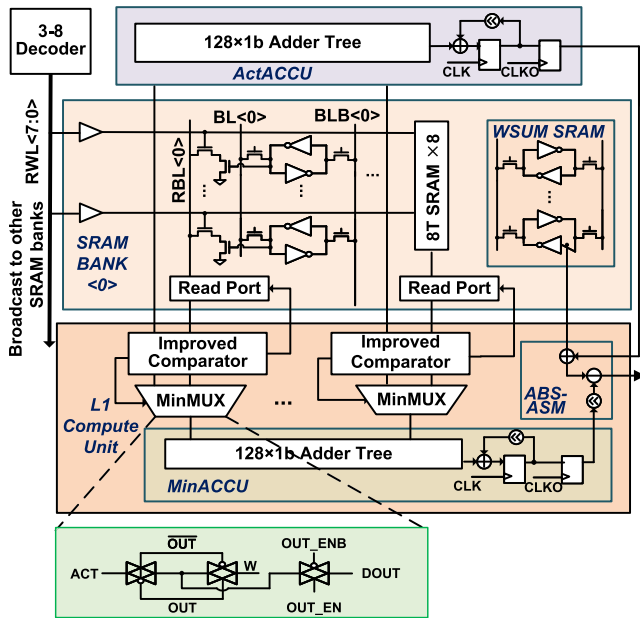
Fig. 8. Circuit-level design and bit-serial computation of L1 compute unit.
