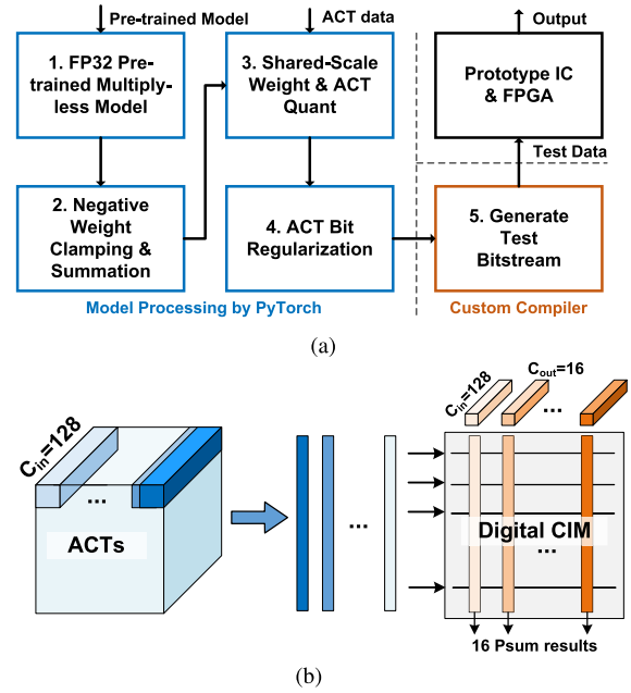
Fig. 18. (a) NN model deployment flow. (b) NN mapping method.
