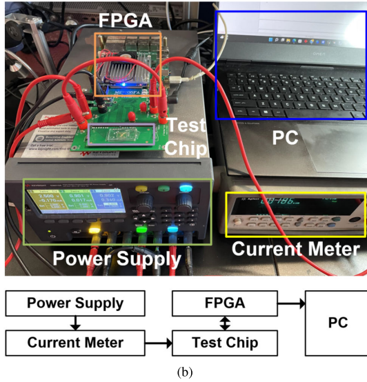
Fig. 14. (a) Chip micrograph. (b) Test platform.
