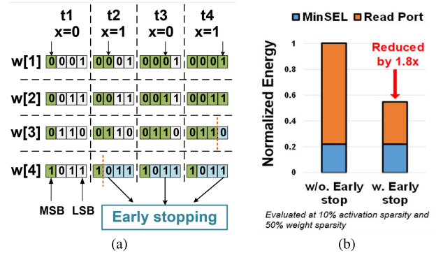
Fig. 10. (a) Early weight-readout stopping mechanism. (b) Read port energy saving for the early stop.
