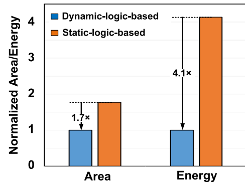
Fig. 12. Area and energy comparison between the static-logic-based comparator and the dynamic-logic-based comparator.
