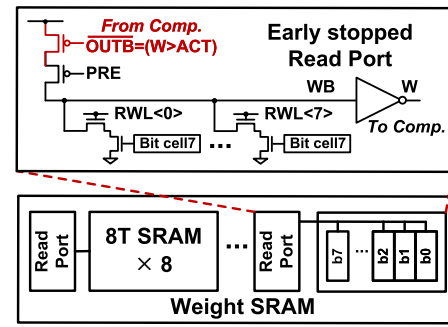
Fig. 9. Schematic of the specialized local SRAM read port.
