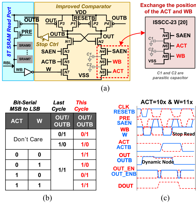
Fig. 11. (a) Schematic of the improved comparator. (b) State transition table for improved comparator. (c) Waveform for comparison operation.
