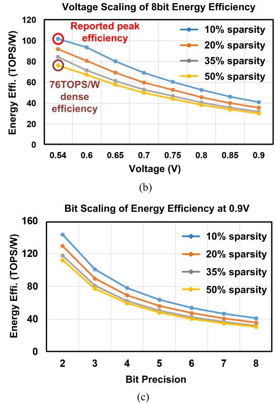
Fig. 15. (a) Voltage–frequency scaling. (b) Voltage scaling of 8-bit energy efficiency. (c) Bit scaling of energy efficiency.
