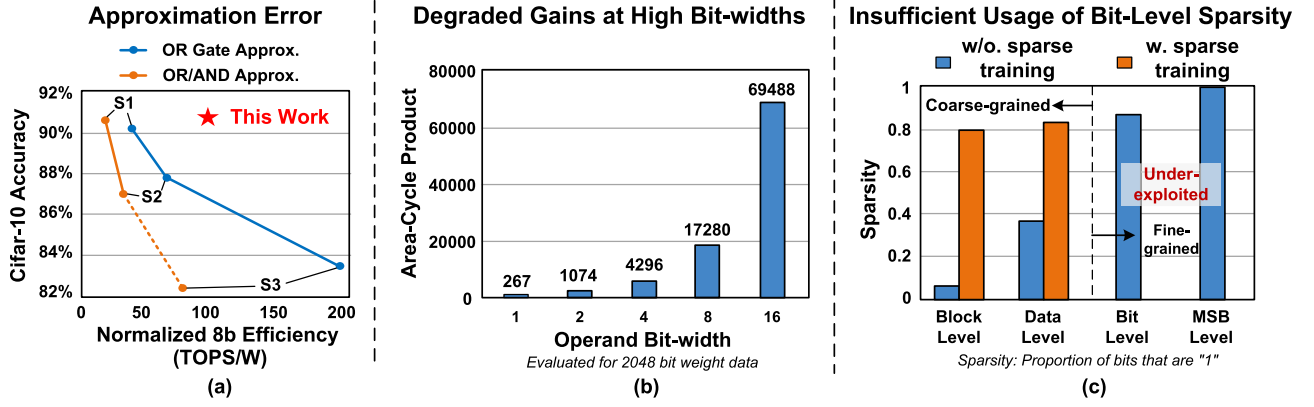
Fig. 2. Three challenges of approximate digital CIM. (a) Approximation error by circuit-level approximation. (b) Degraded gains due to multiplications at high bit-widths. (c) Insufficient use of bit-level sparsity.
